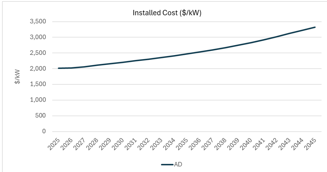
Figure 31. Aeroderivative Turbine Installed Costs
