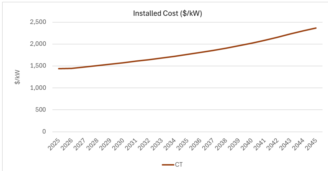
Figure 30. NGCT Installed Costs
