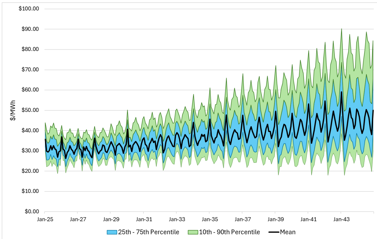
Figure 87. Energy Market Prices Stochastic Results
